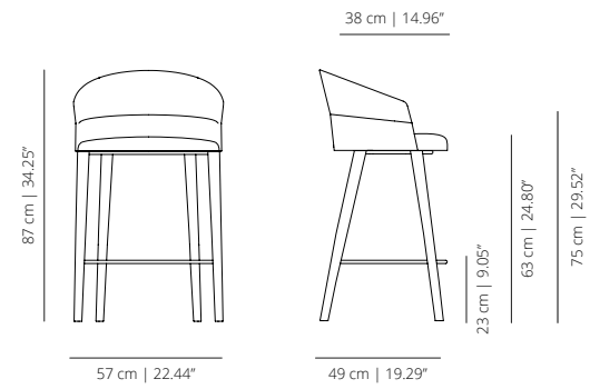
COT4MACO stool
