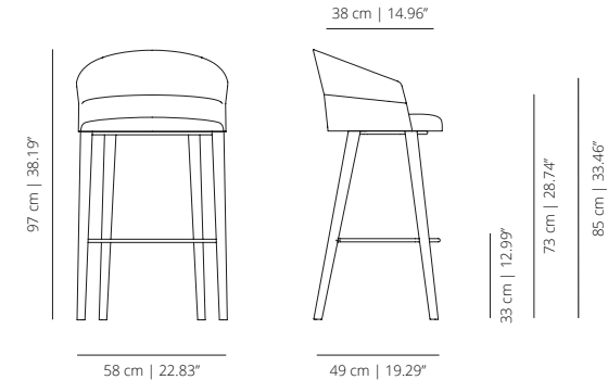
COT4MABAR stool
