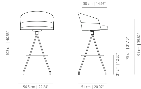
COTGBAR stool
